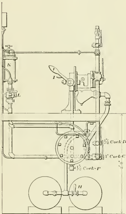
TRIPLE VALVE TESTING MACHINE—END VIEW.
